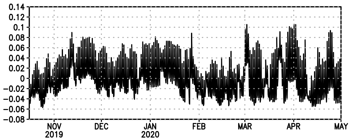
EOF-2 of combination of slp, q2, rh2, t2
