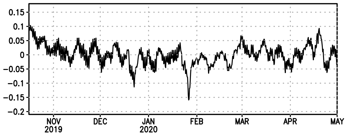
EOF-3 of combination of slp, q2, rh2, t2
