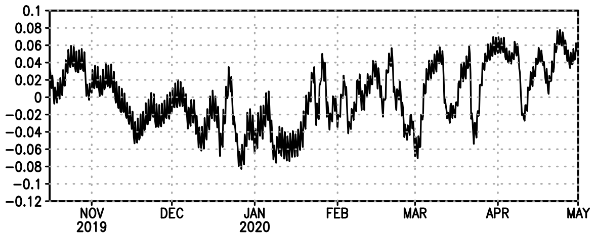
EOF-1 of combination of slp, q2, rh2, t2
