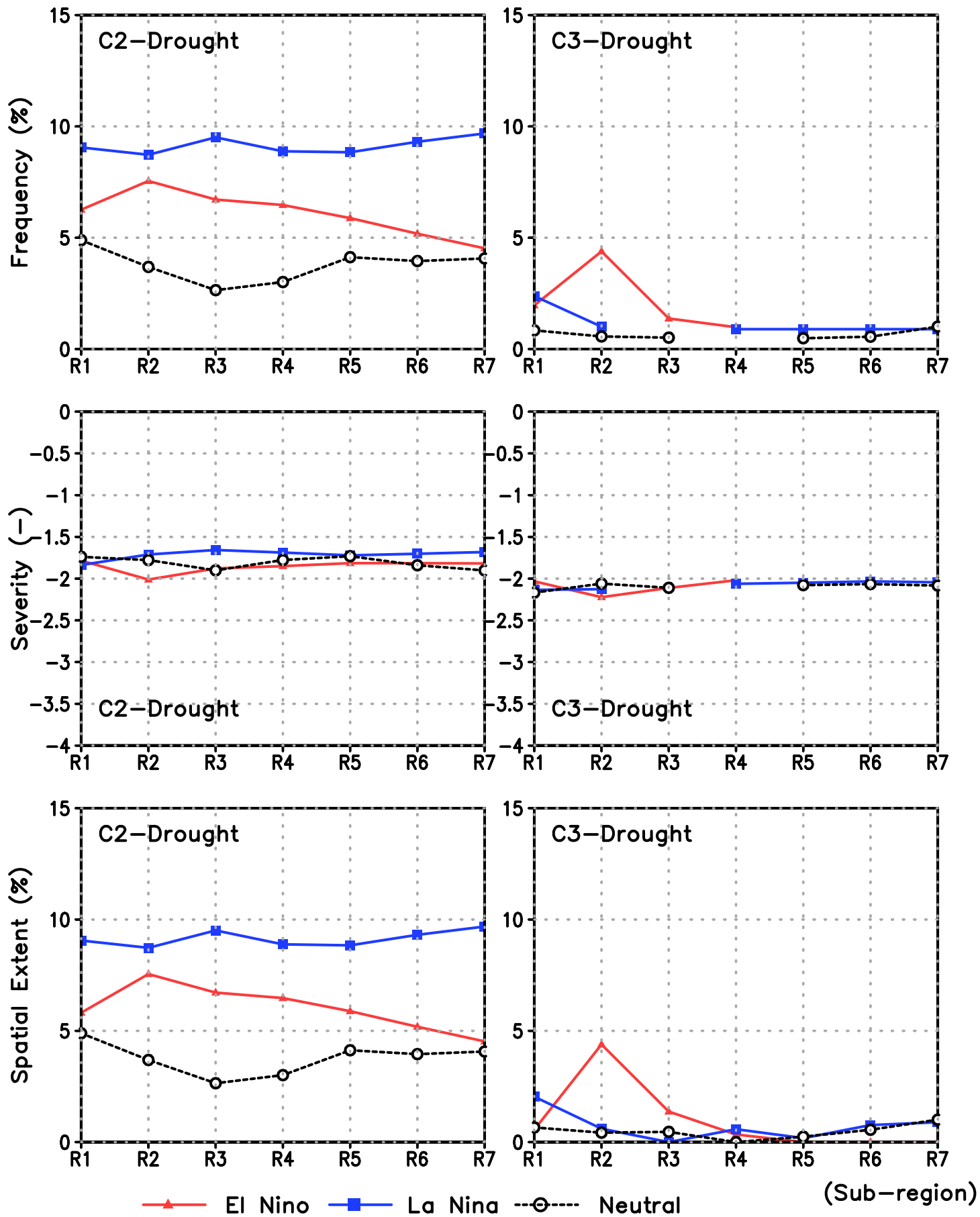
Characteristics of C2– and C3–Drought with respect to ENSO phases over sub-regions (R1–R7)
