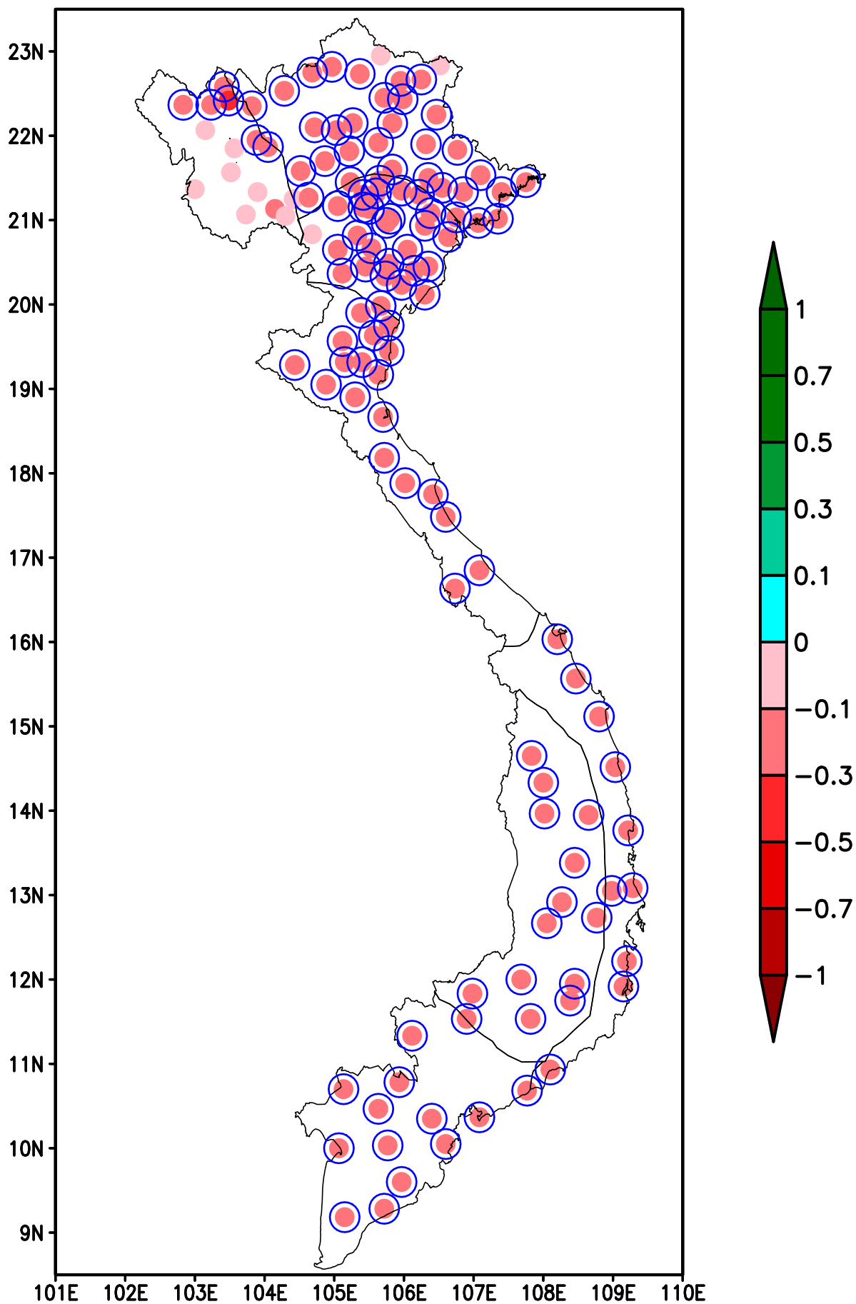
Sens Slopes of PDSI (per decade) (Stations with blue circle: p -value<5%)
