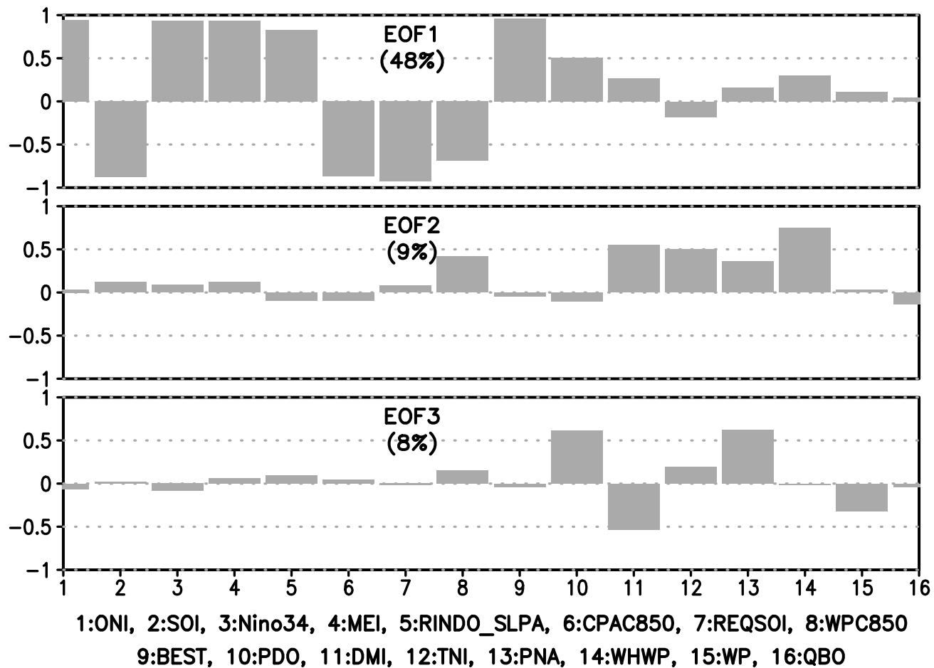
EOFs of 16 selected Climate Indices
