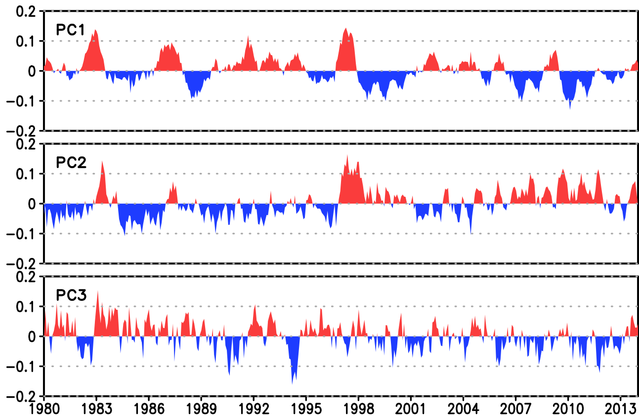
Timeseries of EOFs of 16 selected Climate Indices
