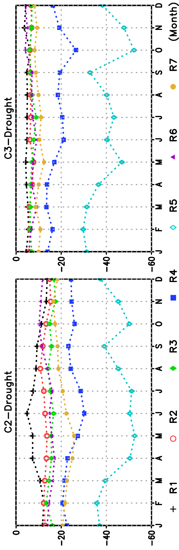
Annual Cycle of Drought Severity (—)
